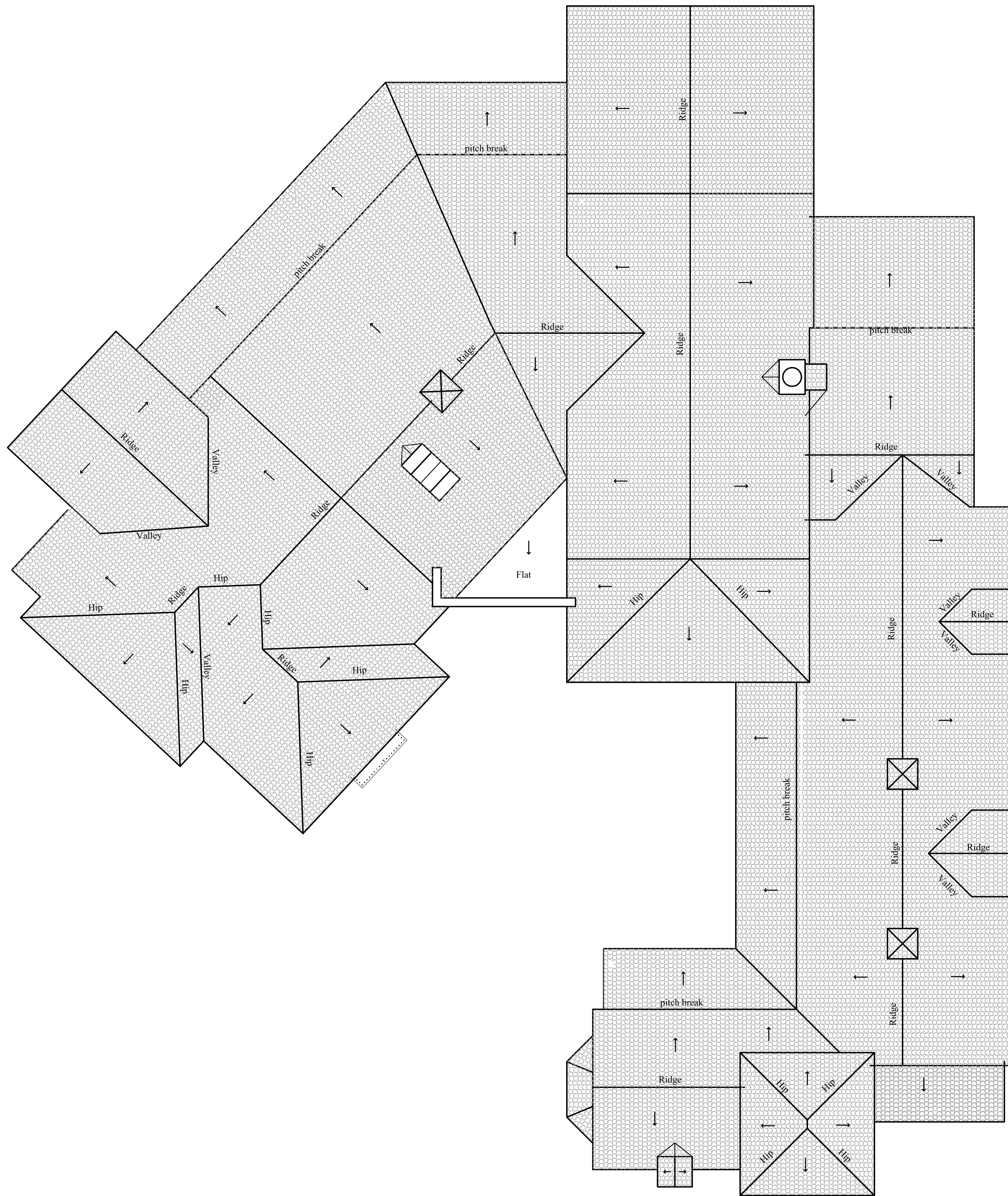
PROPOSED ROOF PLAN 3.5:12 typical pitch u.n.o. 1/8" = 1'-0"
