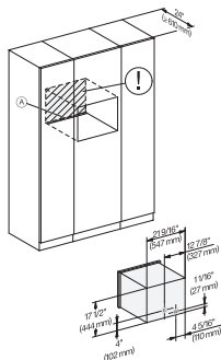
CVA7445, CVA7845, installation drawing, installation, 60 cm, Proud
