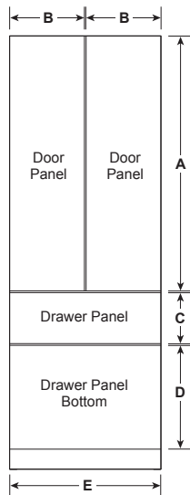
PANEL DIMENSIONS
