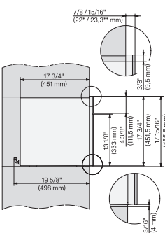
CVA7445, CVA7845, side view, 60 cm, Proud
