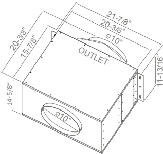
PBN-1000A (in-line)
