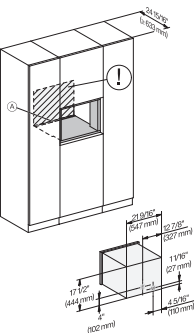
CVA7445, CVA7845, installation drawing, 60 cm, Flush insert
