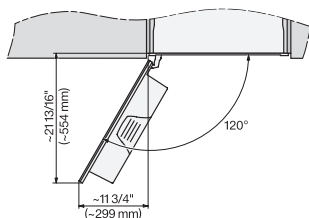
CVA7445, CVA7845, installation drawing, side view, Flush insert
