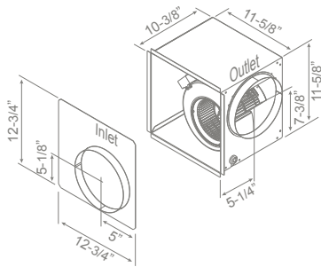
DBI-600A (internal/in-line)
