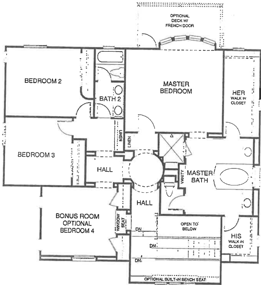
VIRAZON RESIDENCE TWO SECOND FLOOR
