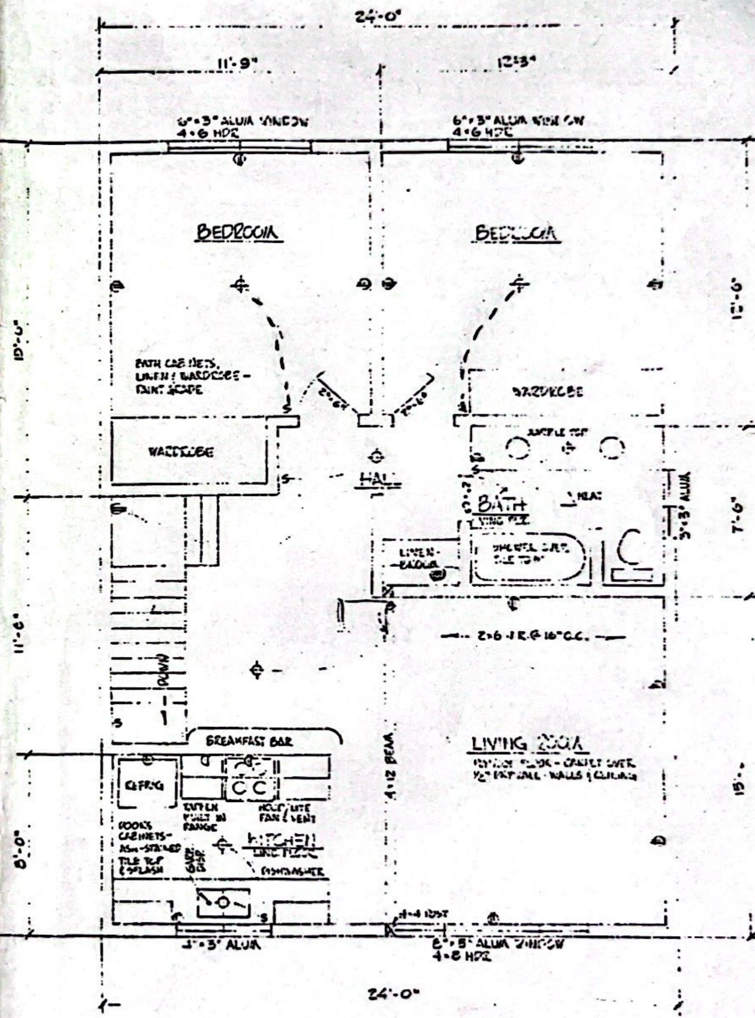
2 nd FLOOR - PLAN A
