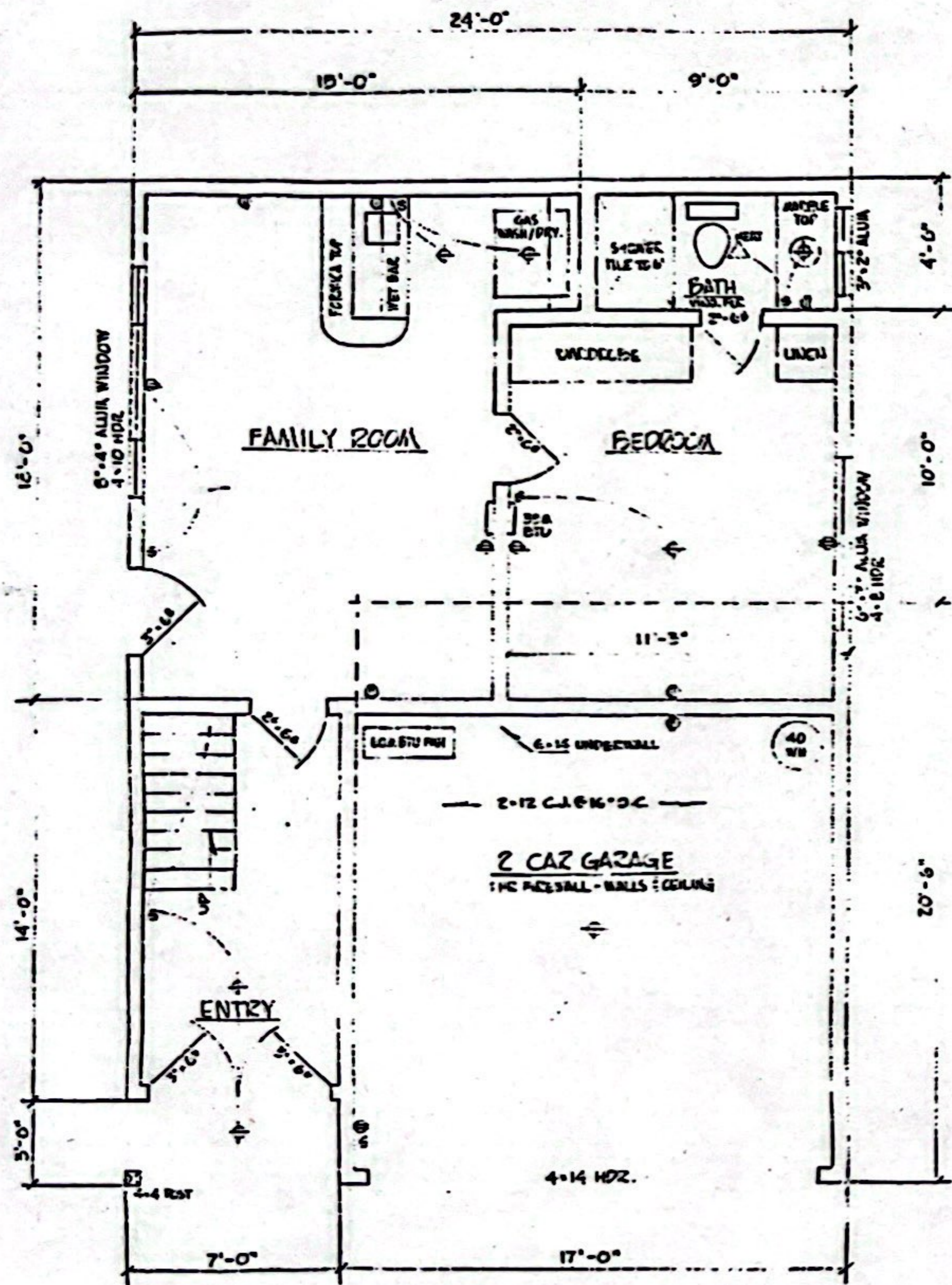
1 st FLOOR - PLAN A
