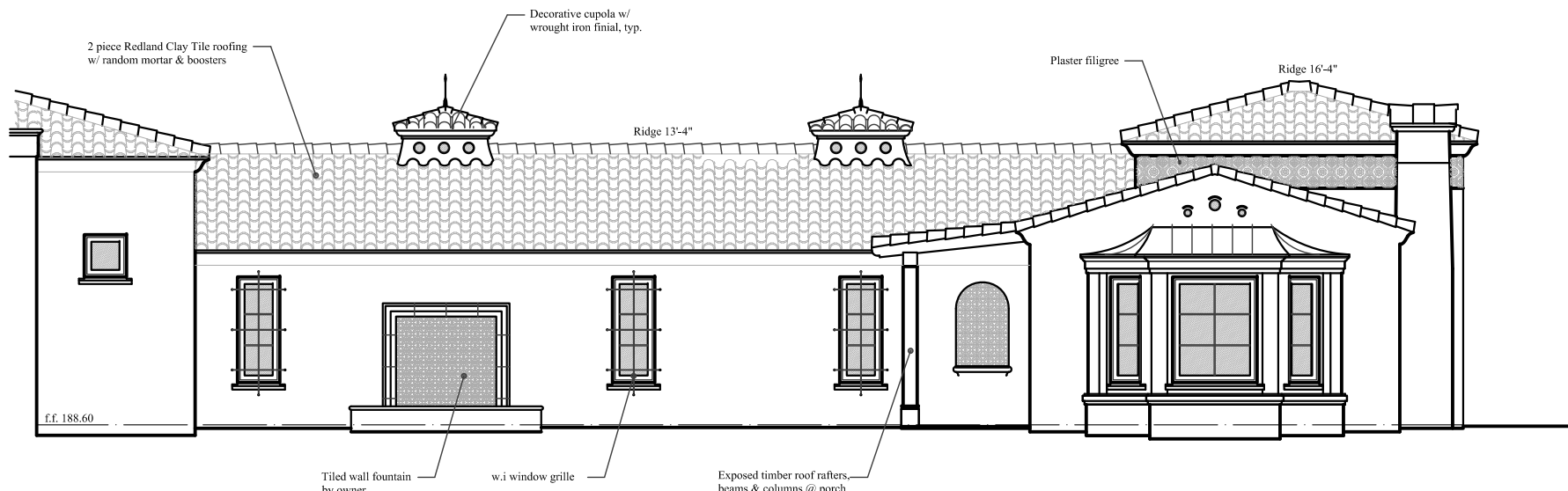
COURTYARD (west) elevation
