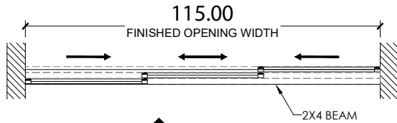
Plan - Closed Position; Scale: None
