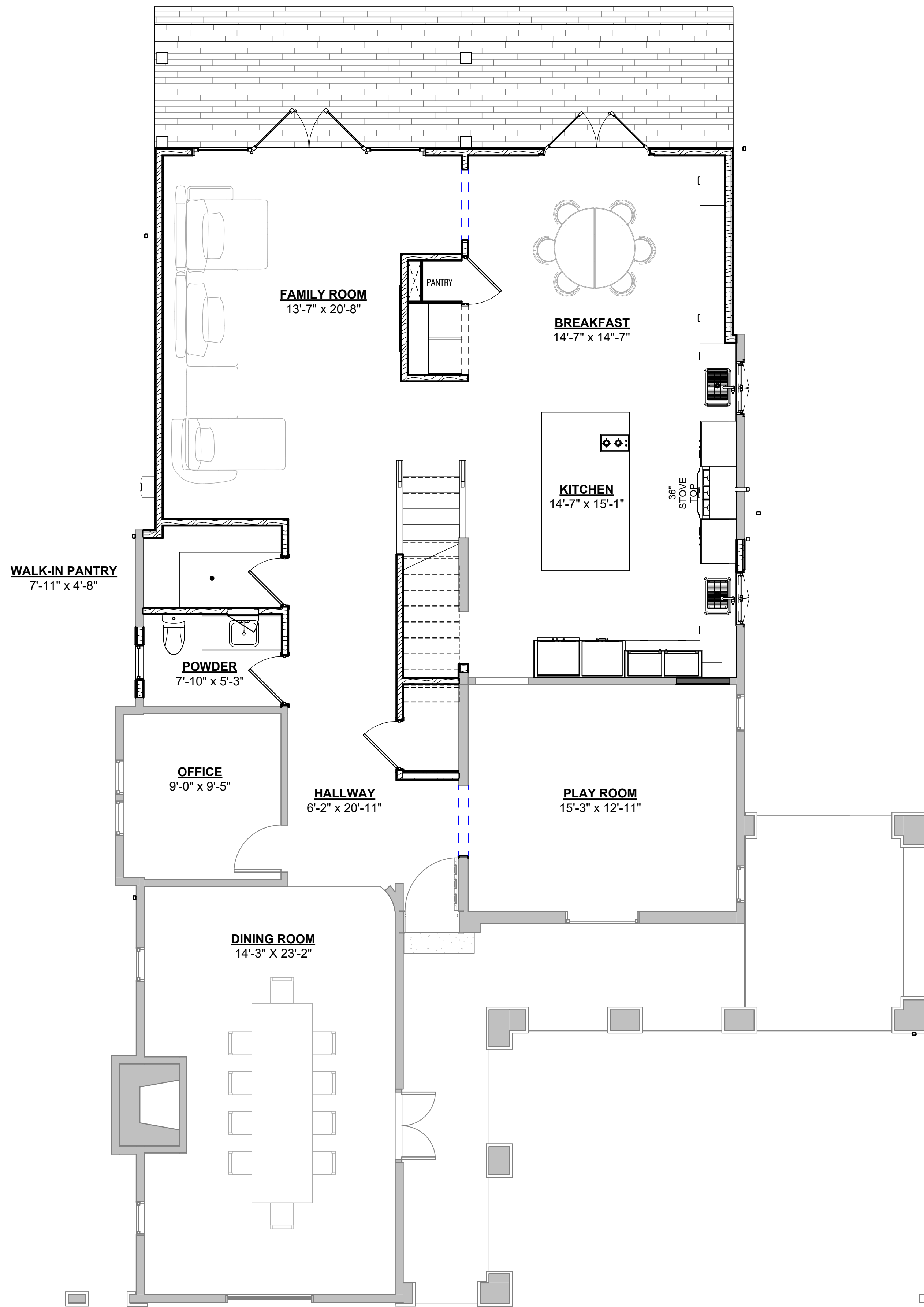
① PROPOSED LEVEL 1 FLOOR PLAN 1/4" = 1'-0"
