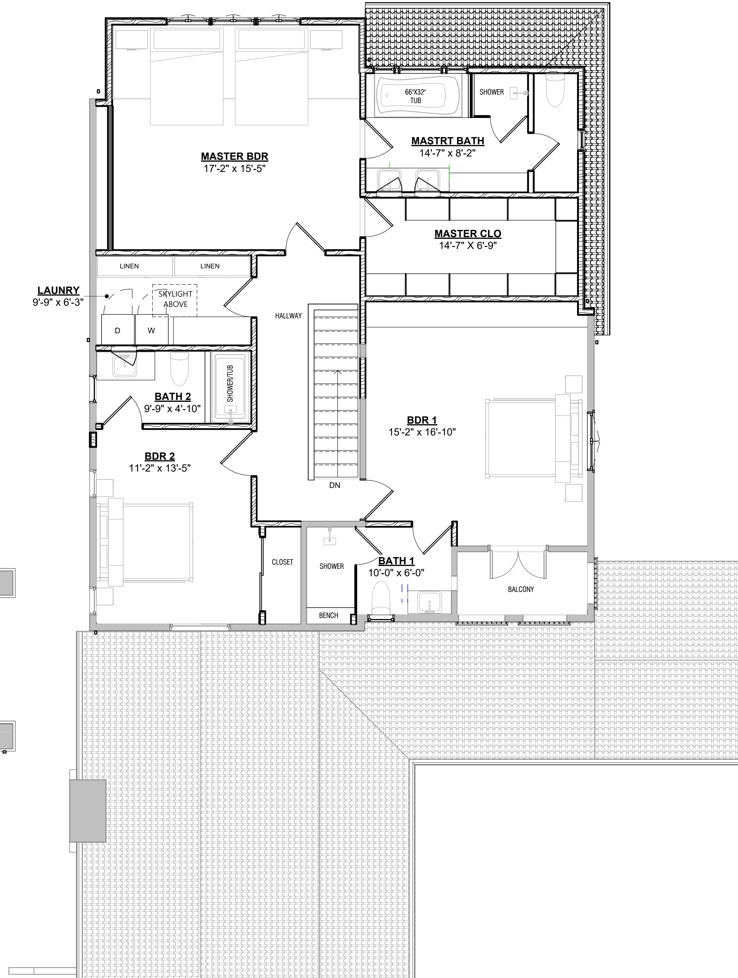
② PROPOSED LEVEL 2 FLOOR PLAN 1/4" = 1'-0"
