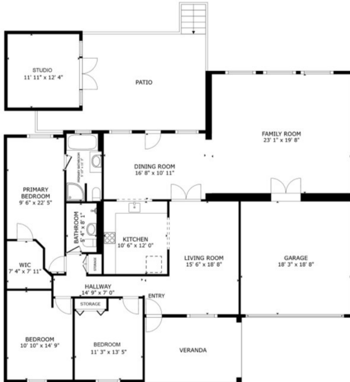
FLOOR PLAN
